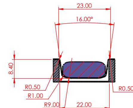
SECTION M-M SCALE 1 : 1
